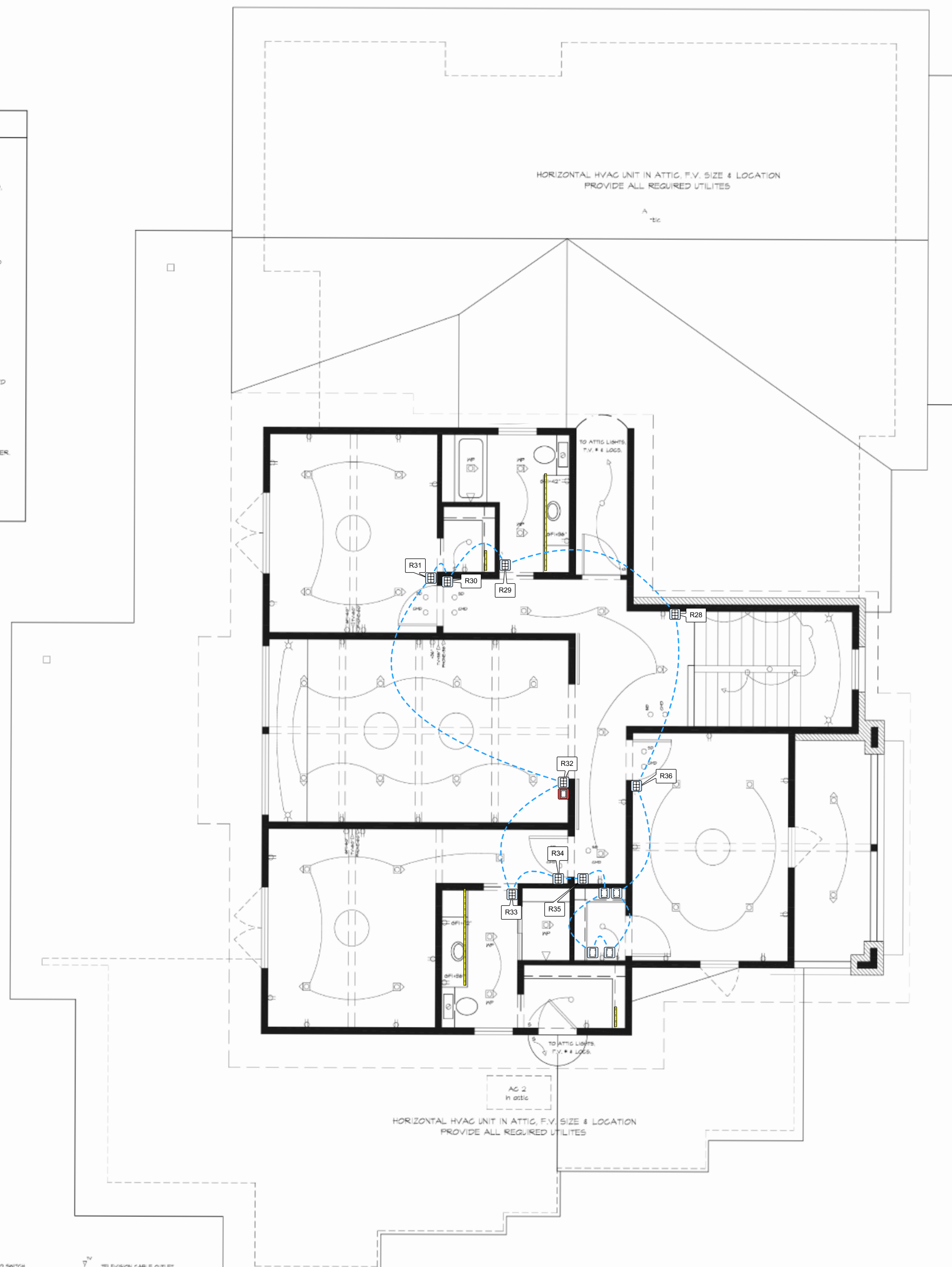
1 UPPER FLOOR ELECTRICAL PLAN SCALE: 1/4" = 1'-0"
